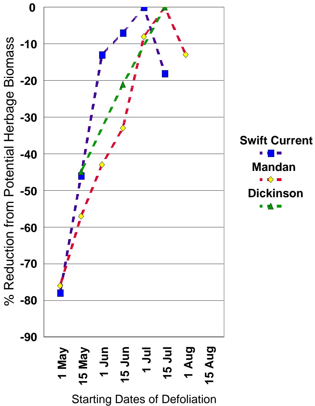
Fig. 1. Percent reduction from potential aboveground herbage biomass on defoliation treatments with different starting dates.
